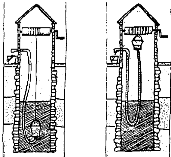
THE HOSE AND BUCKET PUMP
