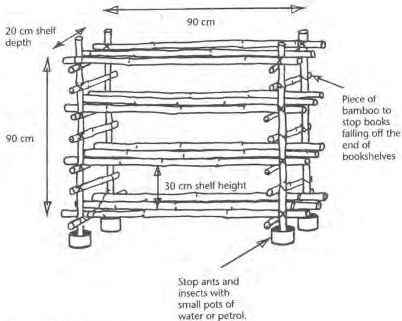
Figure 3.5 Bamboo or loya cane bookshelves
