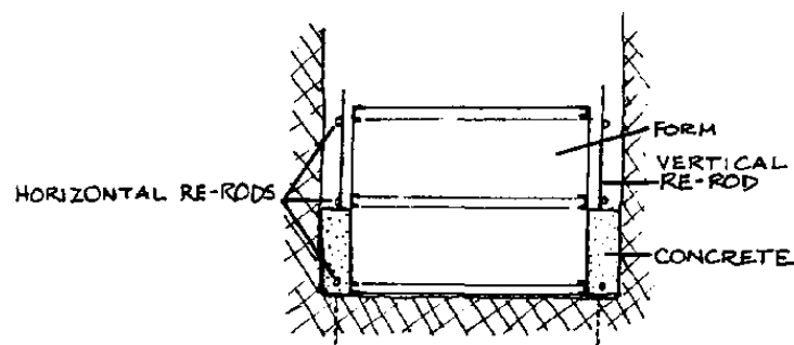
FIG. IV-2. INTERIOR LINING FORM
