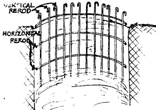
FIG. 8-1. REINFORCED CONCRETE LINING BUILT IN PLACE (a)
