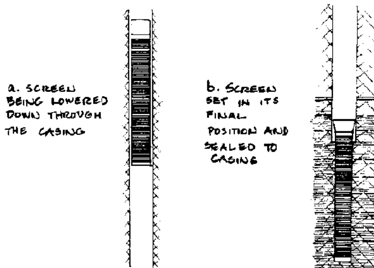
FIG. 15-6. TELESCOPING SCREEN
