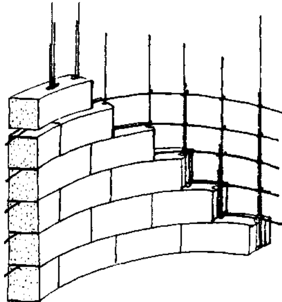
FIG. 8-15. REINFORCED BRICK LINING
