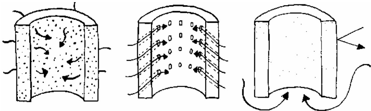
FIG. 3-6. WATER ENTRY INTO WELL
