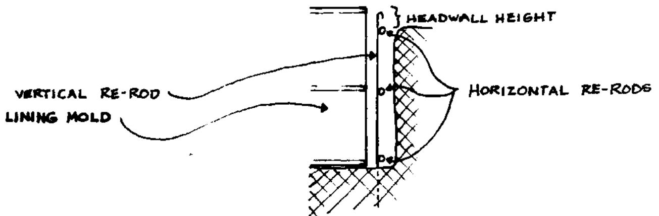
FIG. 8-3. PLACEMENT OF RE-ROD AND FORM IN HOLE
