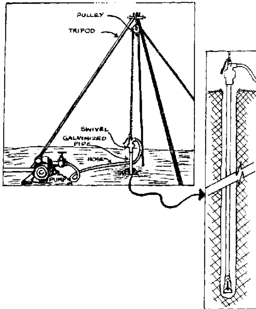
FIG. 11-8. JETTED WELL
