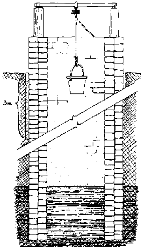
FIG. 8-14. BRICK LINING SUCK ON A CUTTING RING
