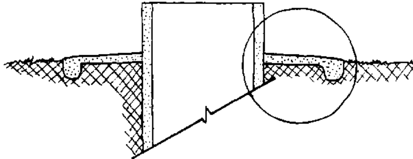
FIG. 3-9. SHALLOW CHANNEL
