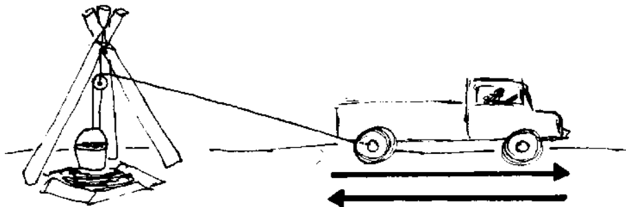
LOWERING/RAISING ROPE ATTACHED TO VEHICLE
