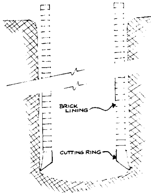
FIG. 8-14. BRICK LINING SUCK ON A CUTTING RING
