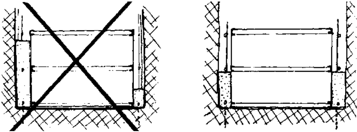
FIG. 8-5. POURING CONCRETE EVENLY IN PLACE AROUND MOLD.
