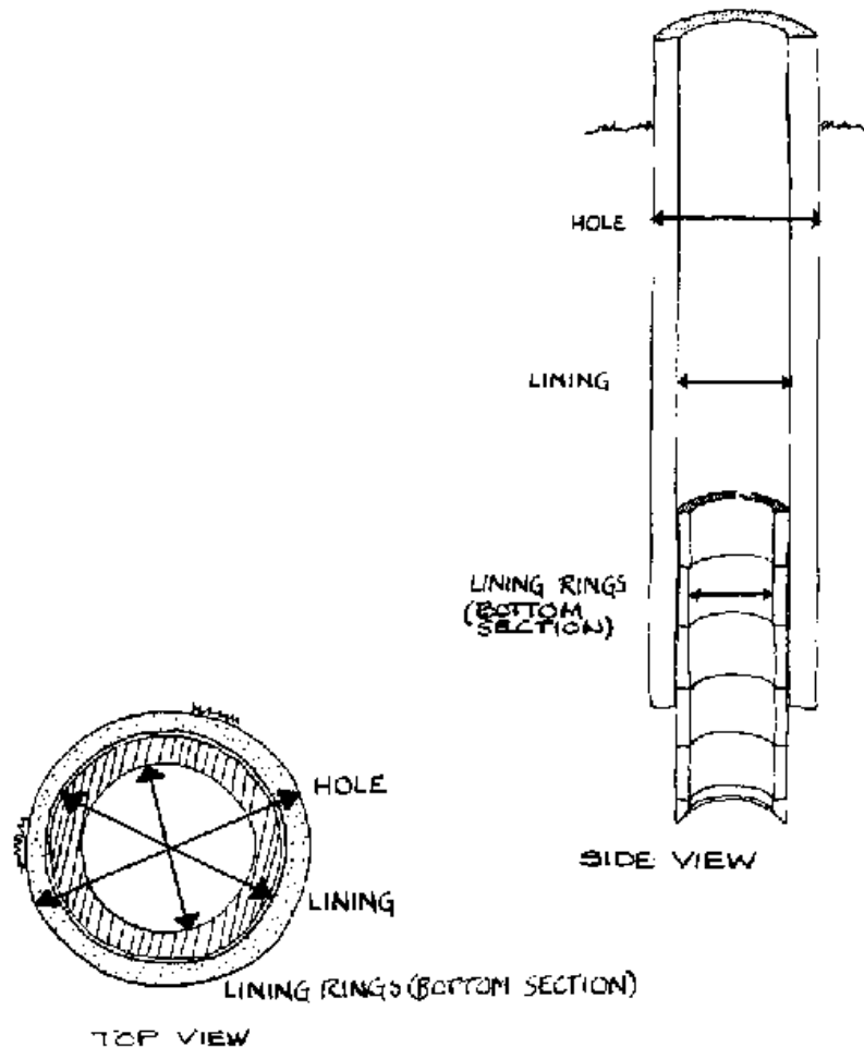
FIG. 3-4. THREE DIFFERENT WELL DIAMETERS USED DURING CONSTRUCTION
