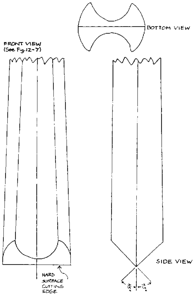
FIG. 12-9. DETAIL OF PERCUSSION BIT
