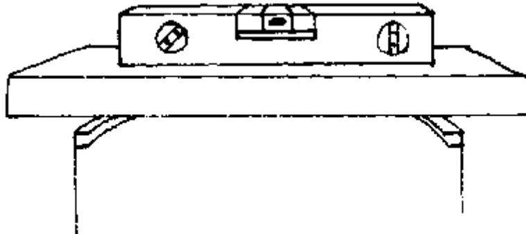
FIG. V-7. USING A STRAIGHT BOARD TO CHECK LEVEL ACROSS MOLD
