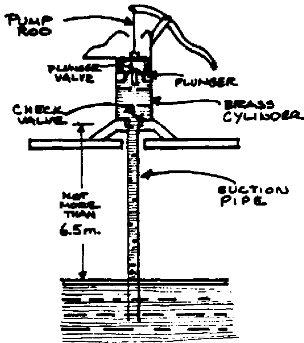
FIG. VII-2. SHALLOW WELL LIFT PUMP
