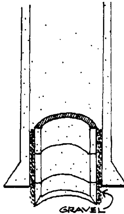
FIG. 9-6. BOARDS USED TO GUIDE SINKING RINGS
