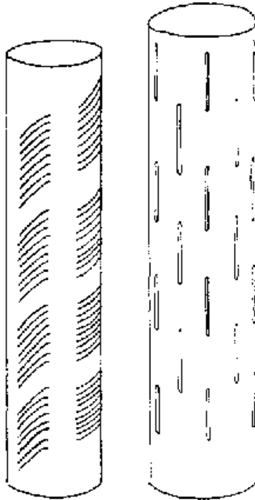
FIG. 15-2. LOCALLY MADE SLOTTED PLASTIC PIPE
