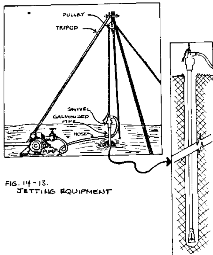
FIG. 14-13. JETTING EQUIPMENT
