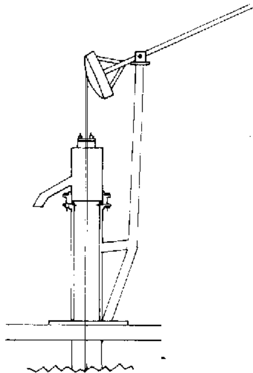
FIG. VII-8. LOCALLY MADE VARIATION OF JALNA PUMP
