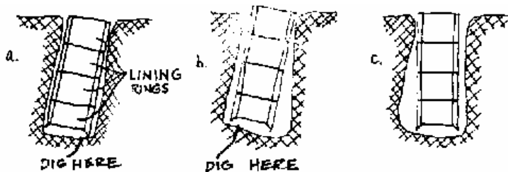
FIG. 8-11. STRAIGHTENING A COLUMN THAT HAS BEEN SUNK OUT OF PLUMB
