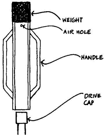
FIG. 14-7. STEEL DRIVING BAR ARRANGEMENT
