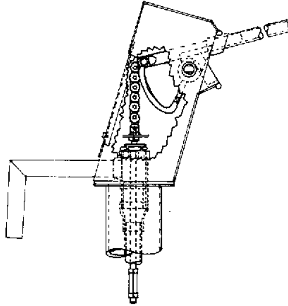
FIG. VII-8. LOCALLY MADE VARIATION OF JALNA PUMP
