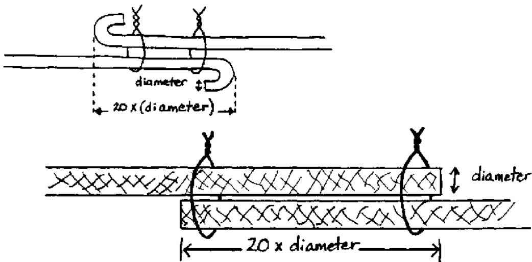
FIG. IV-4. REROD OVERLAP
