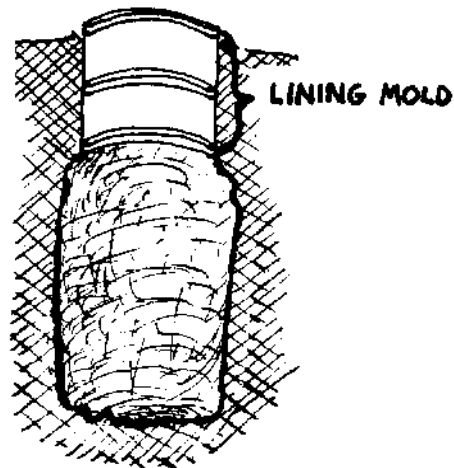
FIG. 7-5 LINING MOLD AS TEMPORARY LINING
