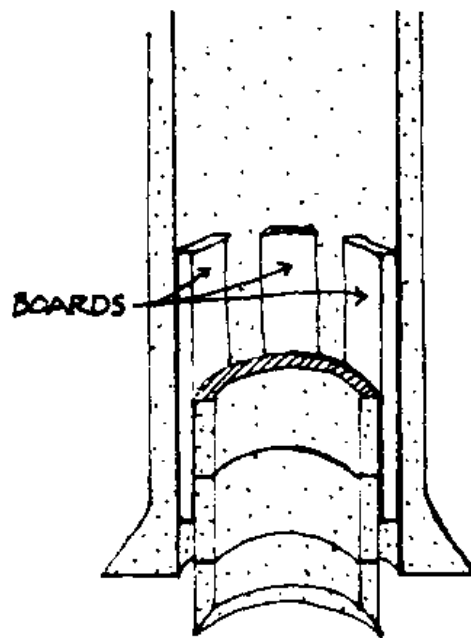
FIG. 9-6. BOARDS USED TO GUIDE SINKING RINGS
