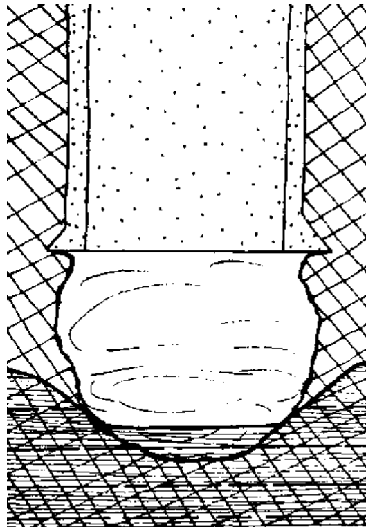
FIG. 9-2. HOLE WALLS COLLAPSING IN BOTTOM SECTION
