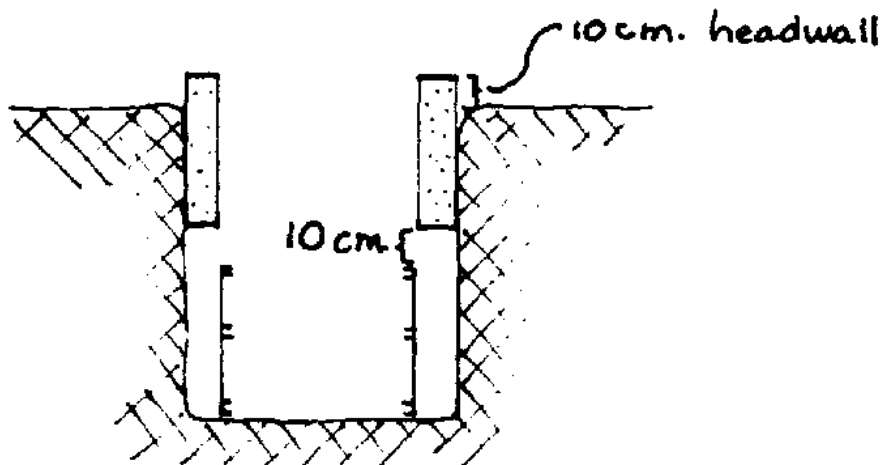
FIG. 8-6. PROPER HOLE DEPTH BENEATH AN ALREADY POURED LINING SECTION
