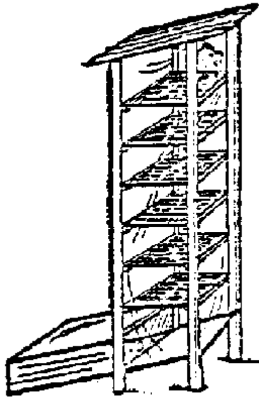
Fig. 18 Improved air-dryer for cocoa and coffee, Sierra Leone
