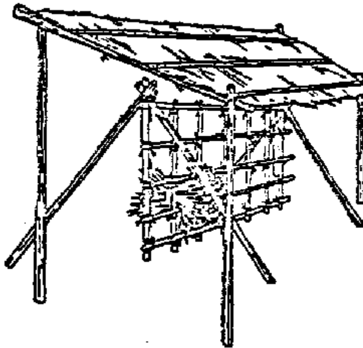
Fig. 9 Fish smoker, Ivory Coast
