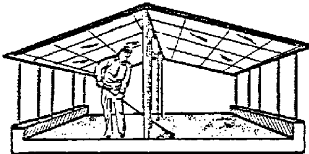
Fig. 22 Plastic-covered, walk through solar coffee dryer, Columbia
