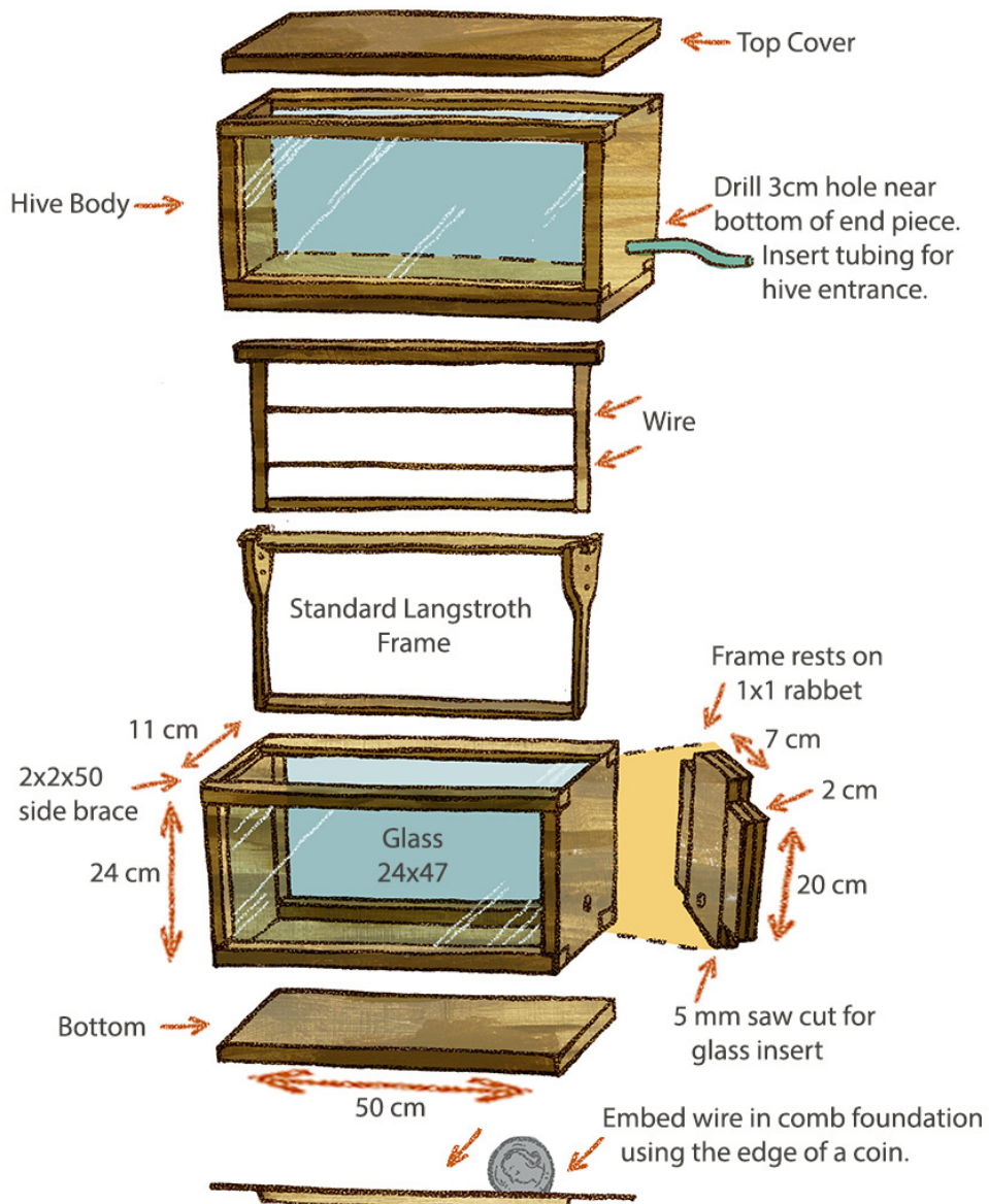
Figure 5-1: Observation Hive
