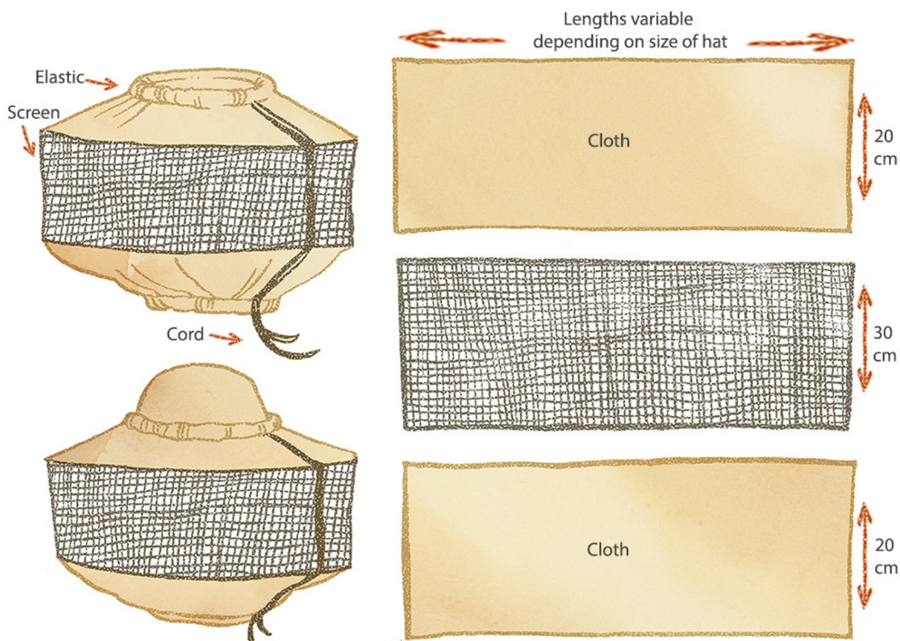
Figure 8-1: Veil Dimensions
