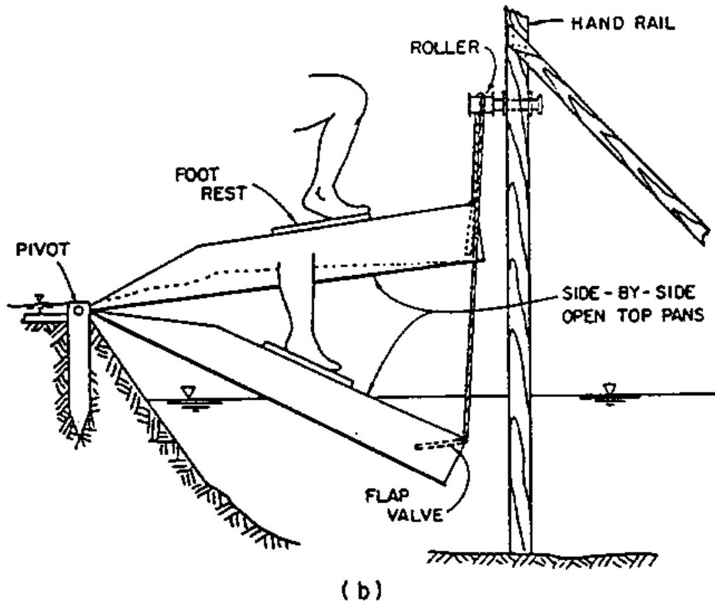
Figure 3.24 Self- Emptying Not with Inclined Tow Path (Ref. 58)
