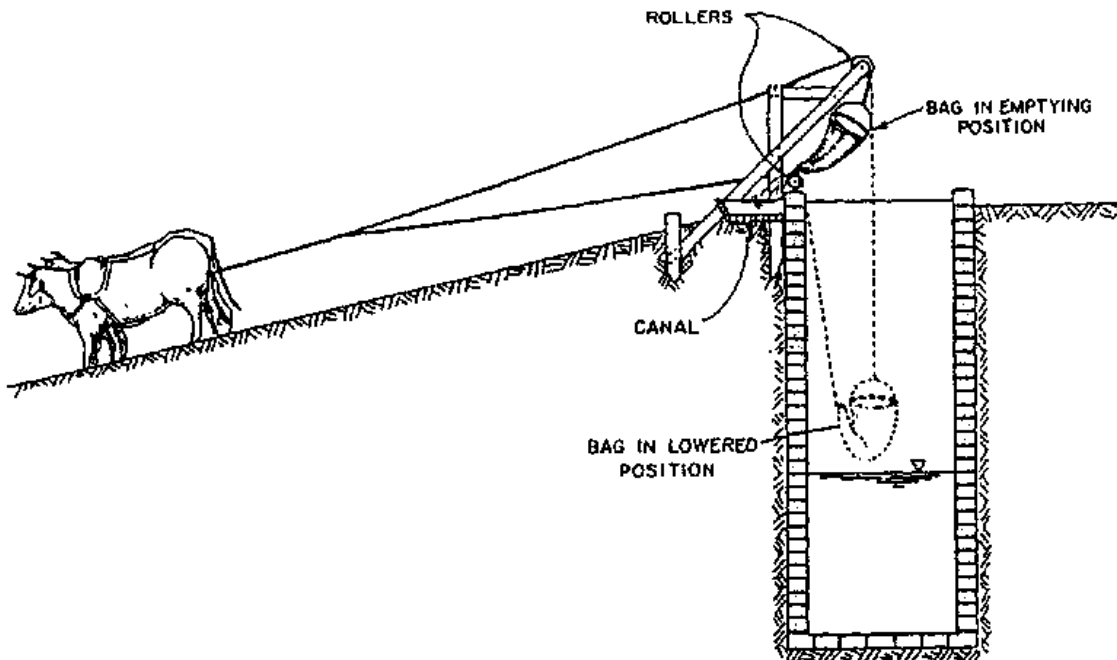
Figure 3.25 Rower Pump (Ref. 28)
