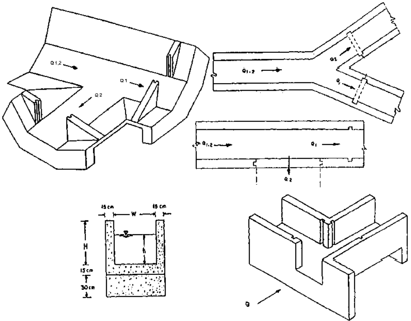
Figure 5.12 Flow Dividers
