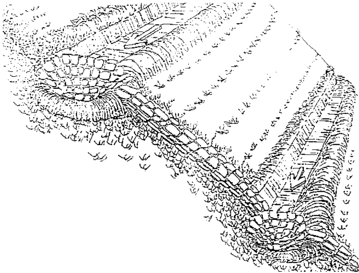
Figure 2.11 Retention Well as a Site for Diverting Runoff eater (Ref. 9)
