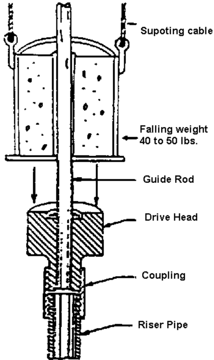
cross-section of sliding hammer and drive stem
