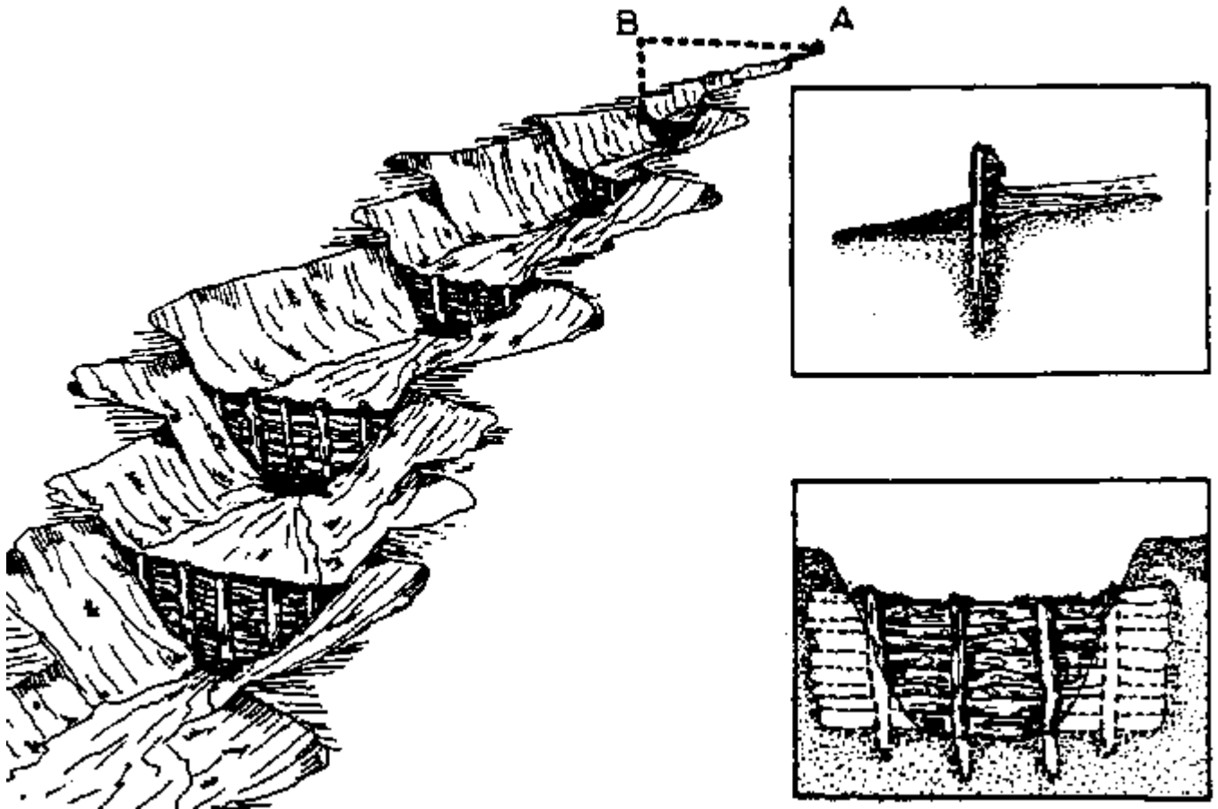
Figure 2.8 A Woven Wire Check Dam
