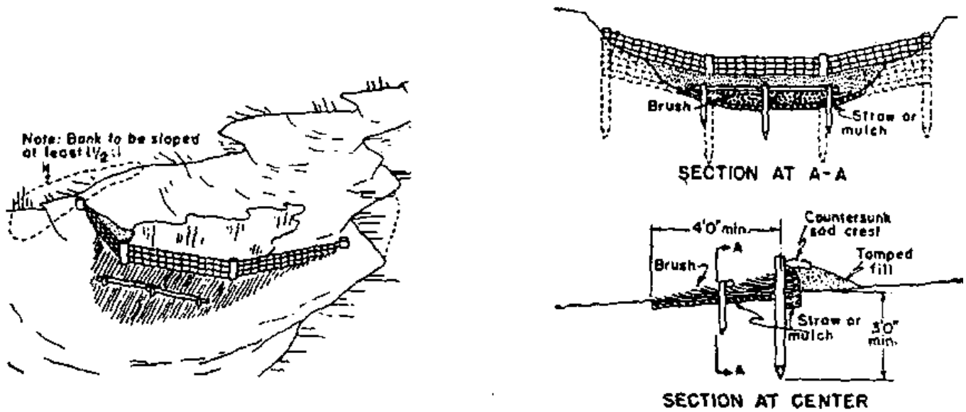
Figure 2.8 A Woven Wire Check Dam
