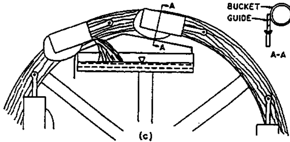
Figure 3.19 Modified Persian Wheel or Zawafa (Ref. 58) (a)
