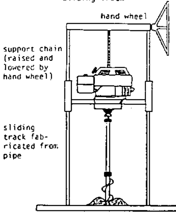
Rotary Engine Mounted on a Sliding Track
