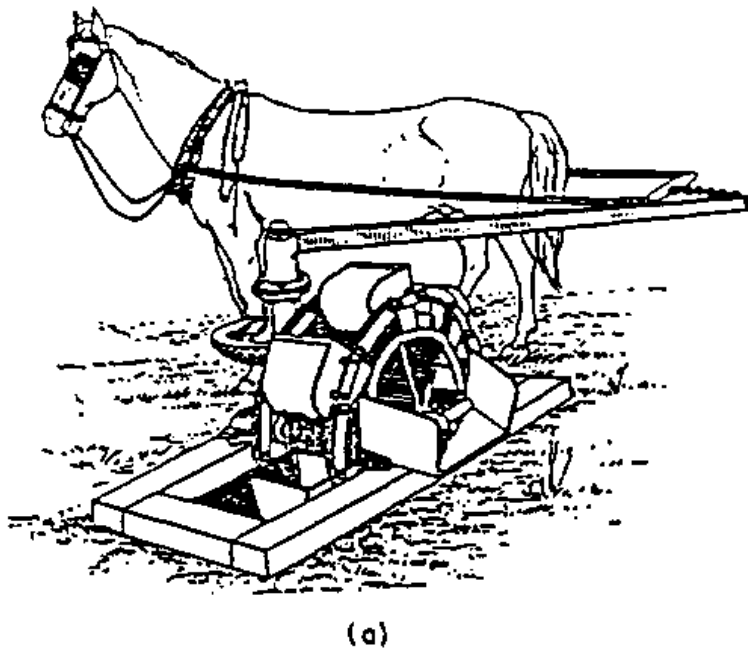
Figure 3.19 Modified Persian Wheel or Zawafa (Ref. 58) (b)
