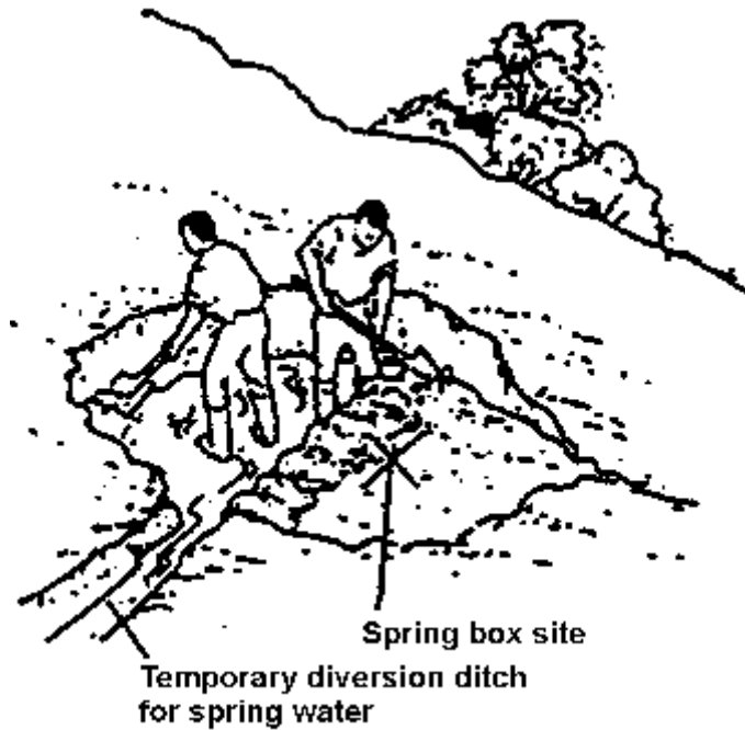
Figure 3.6 Excavating Spring Site (Ref. 39)
