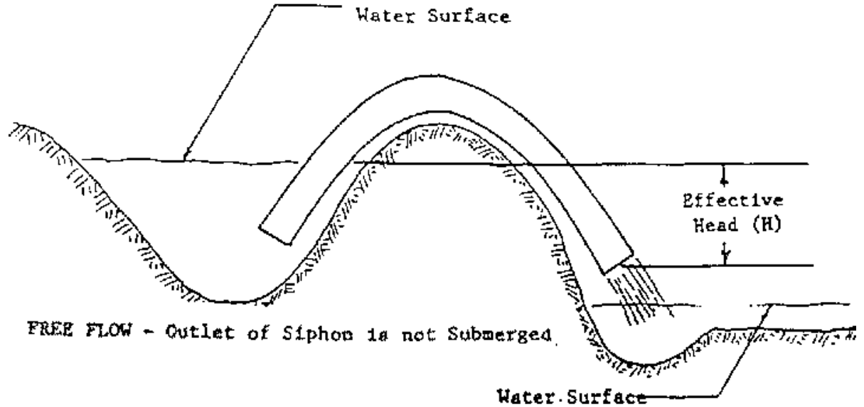
Figure 2.23 Siphon Tubes: Bead Measurement and Discharge
