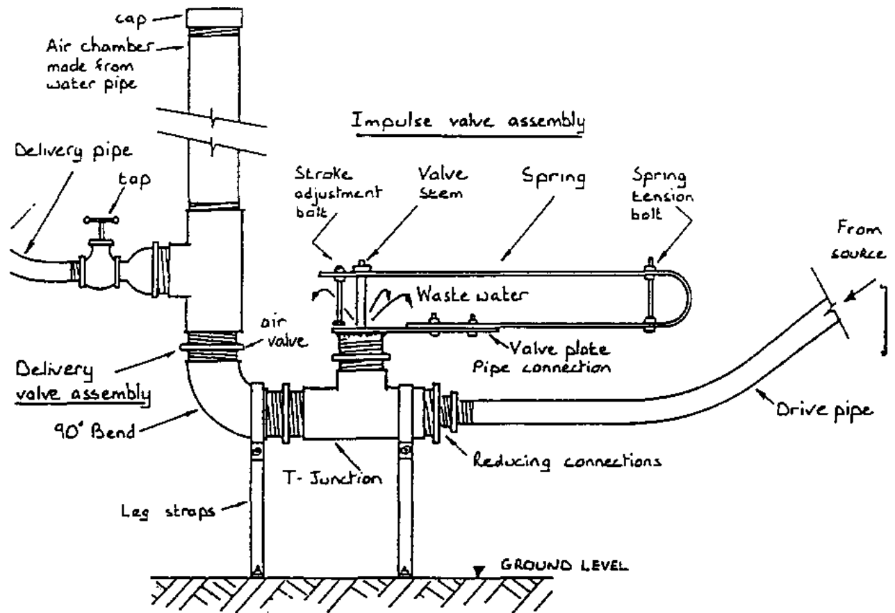
Figure 3.37 Hydraulic Ram (Ref. 55)
