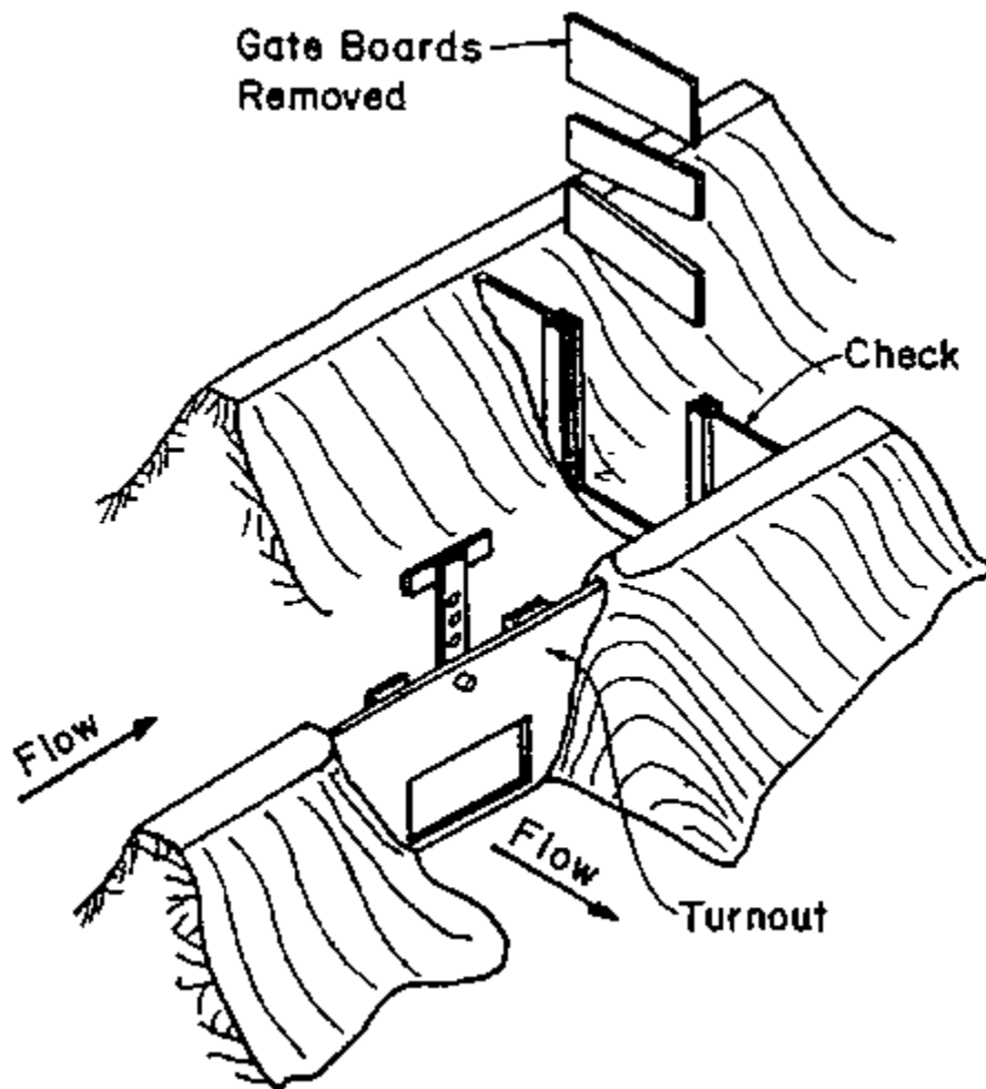
Figure 5.11 Turnout Structures
