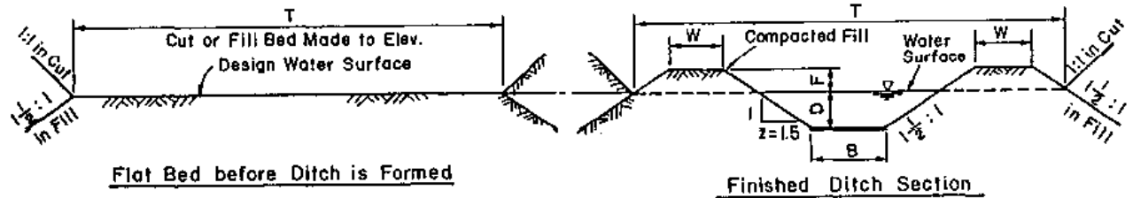
Figure 5.3 Earth Irrigation Ditch Sizes for Different Slopes, Roughness, and Discharges (Ref. 41)
